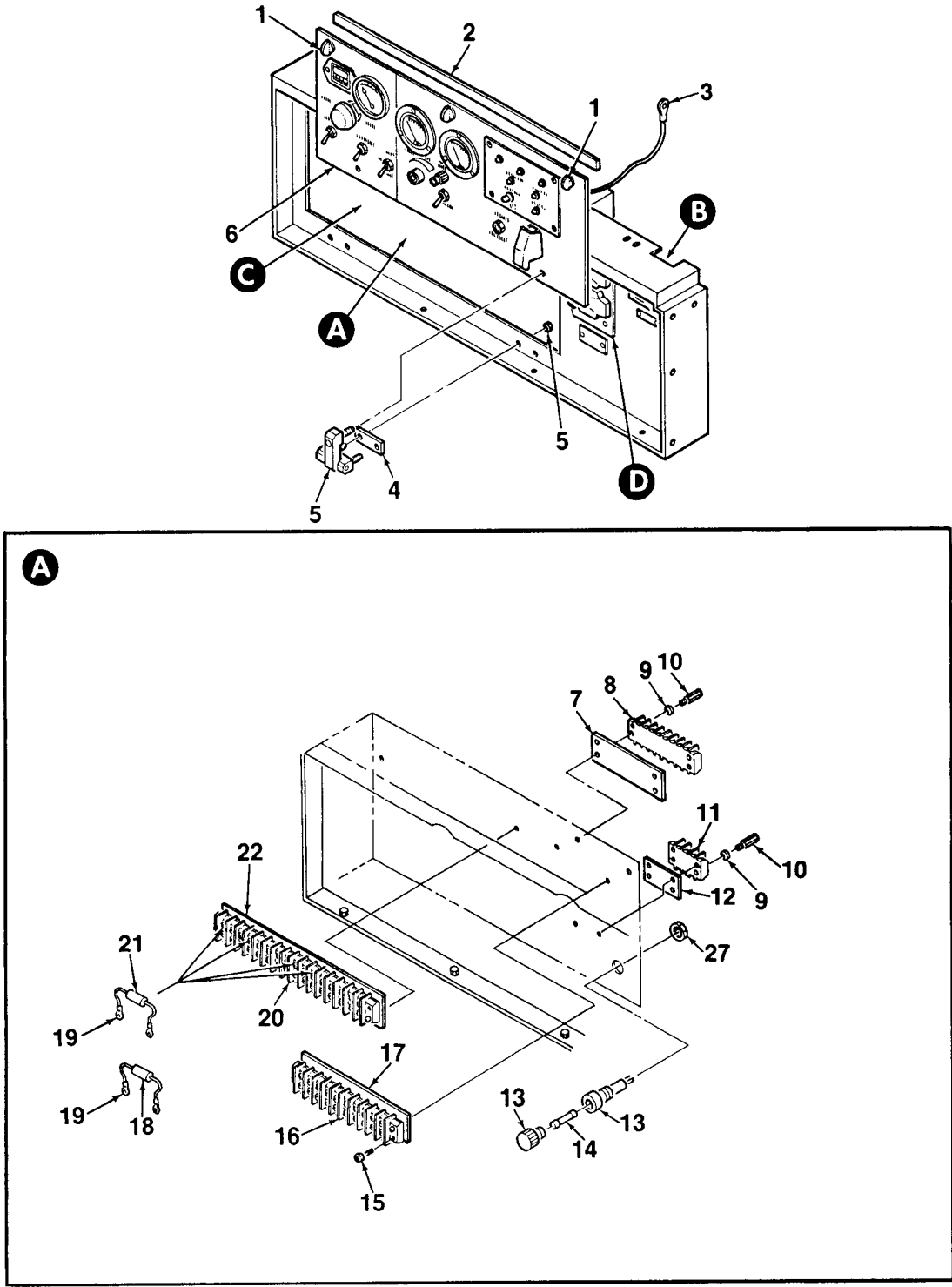
Figure 3. Control Box Assy (Sheet 1 of 3)
