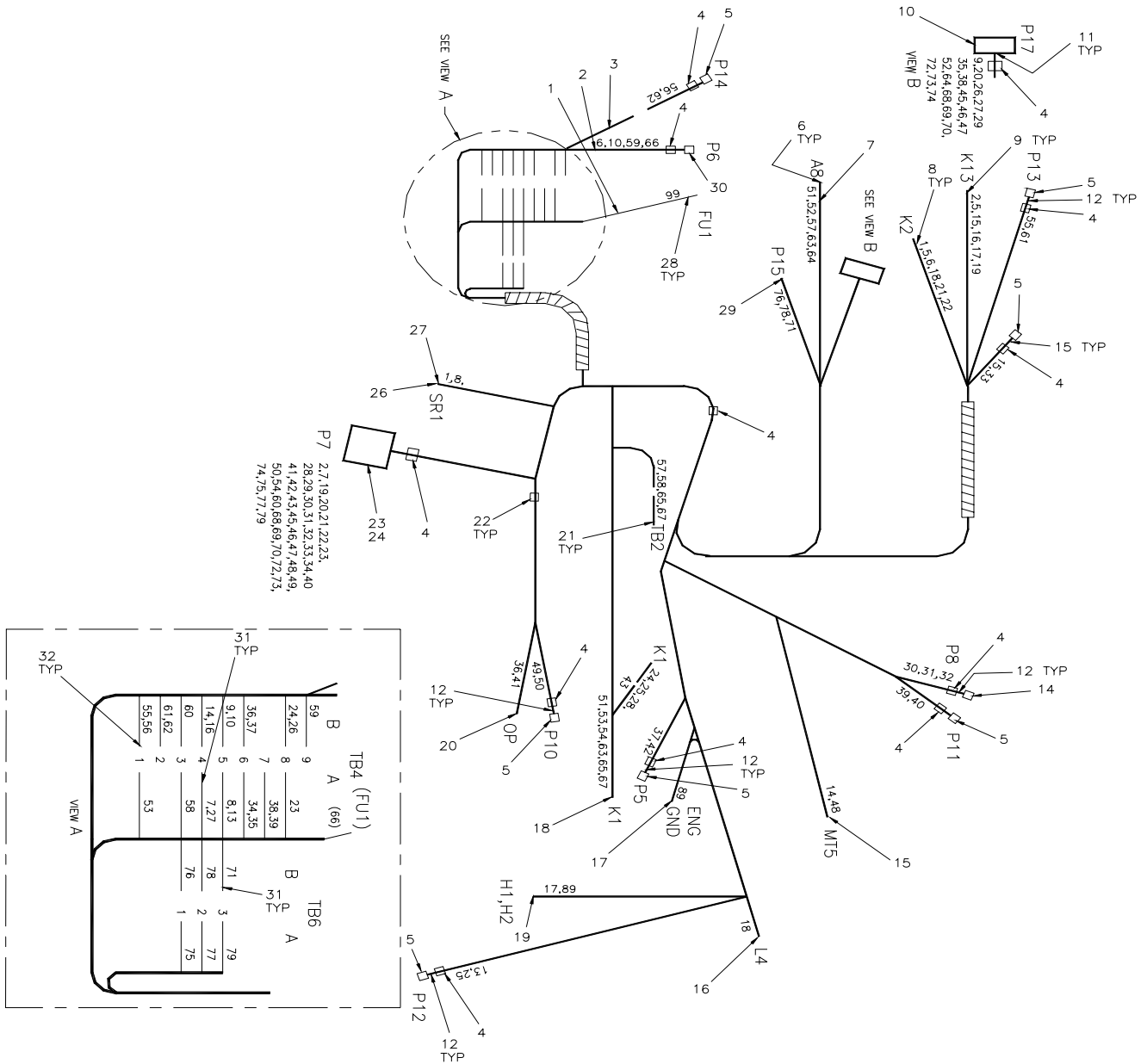
Figure 13. Wiring Harness, Generator Set
