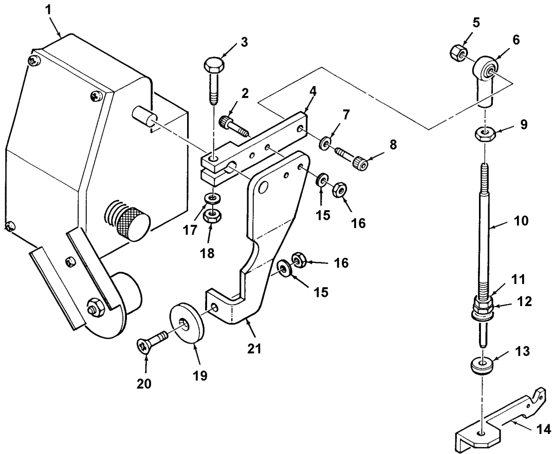
Figure 11. Actuator Assy
