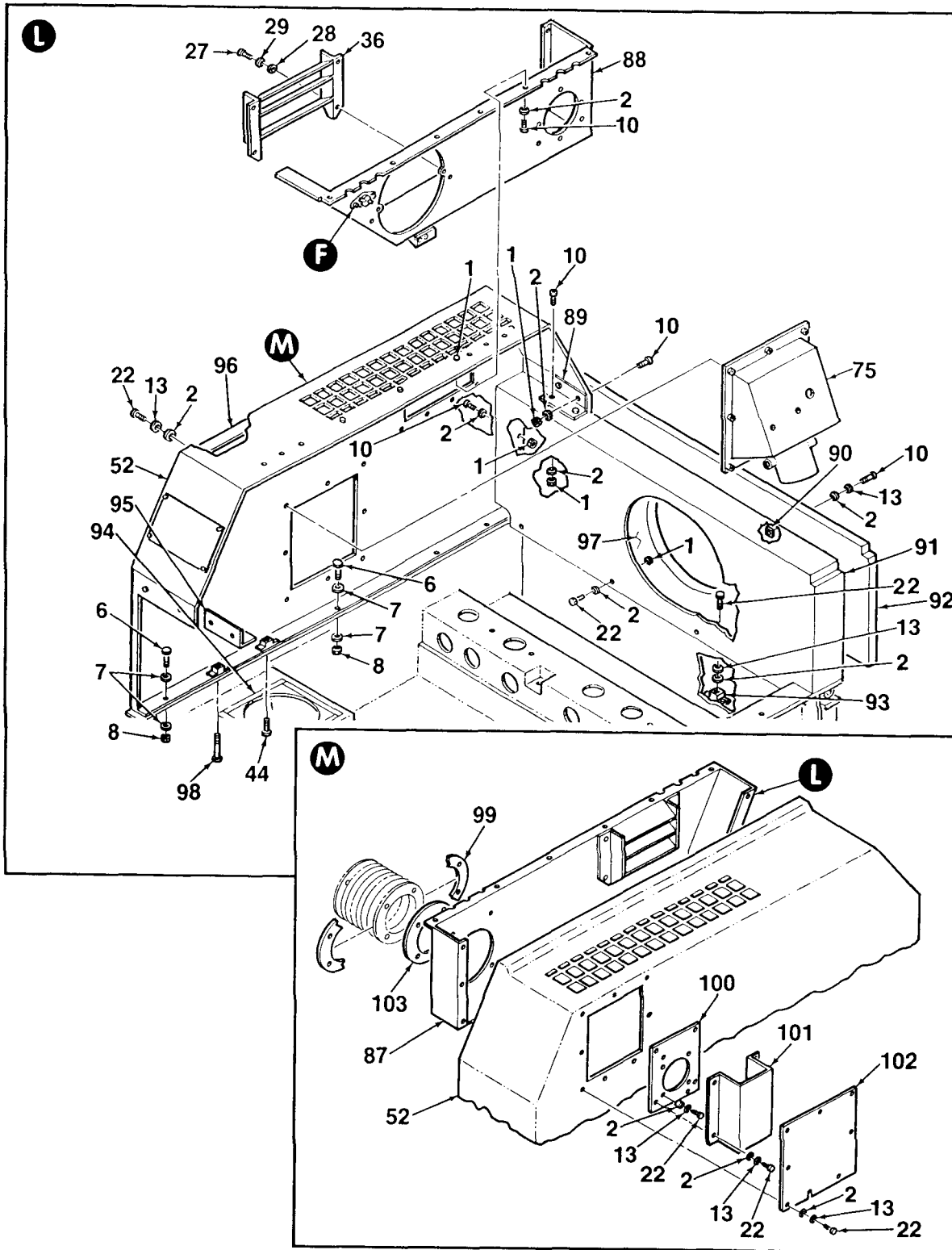
Figure 2. Generator Set Assembly (Sheet 5 of 7)
