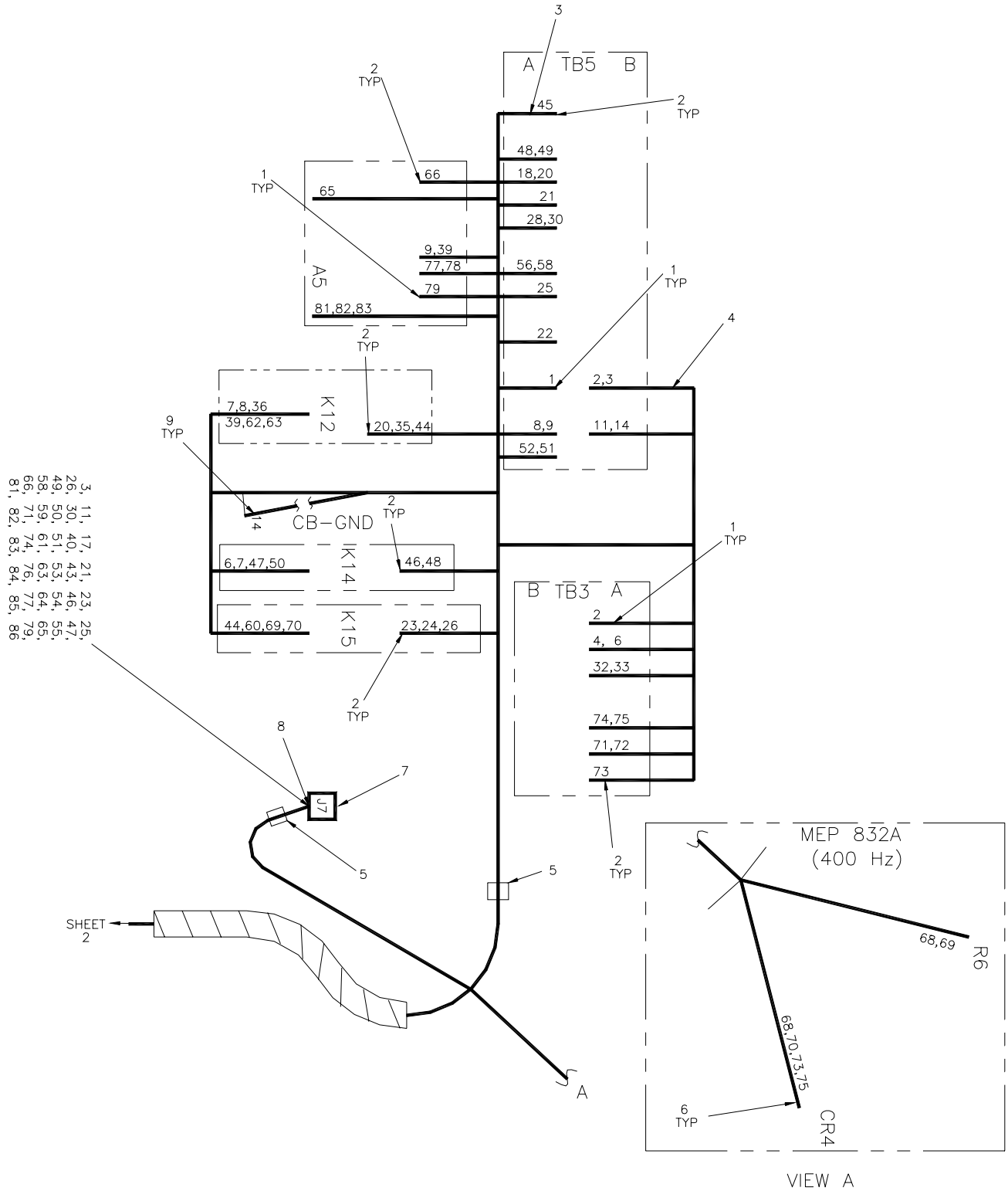
Figure 6. Wiring Harness, Control Box (Sheet 1 of 2)
