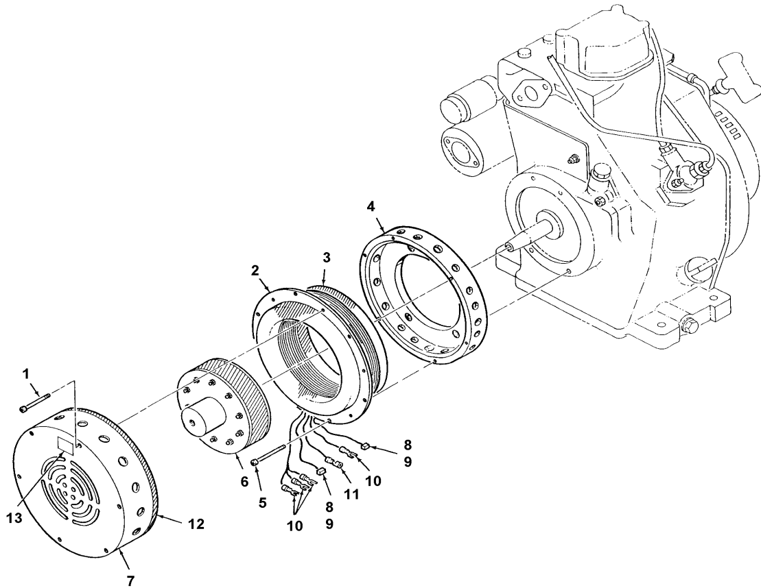
Figure 8. Alternator, Permanent Magnet, 3KW
