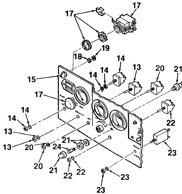
Figure 5. Control Panel Assy
